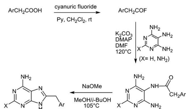
Scheme 1. Three-step synthesis of 8-arylmethyl-9H-purin-6-amines.
