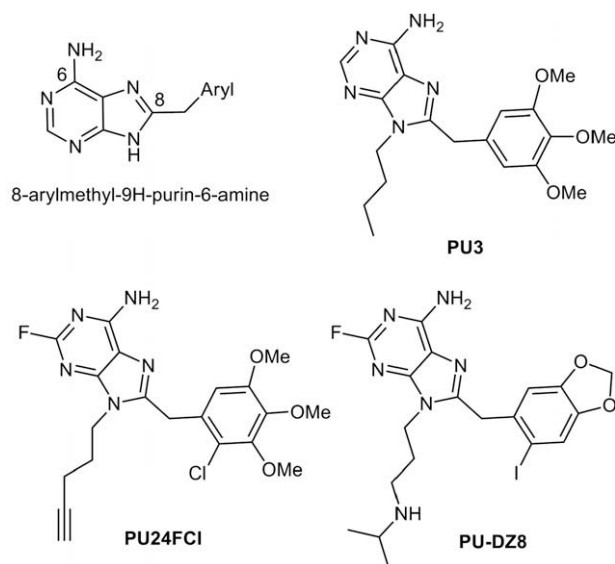
Figure 1. Hsp90 inhibitors containing the 8-arylmethyl-9H-purin-6-amine core.
